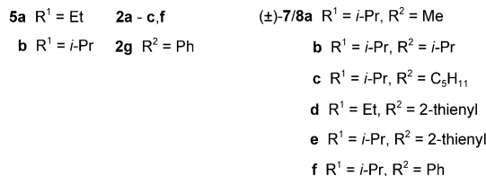
Scheme 3. Preparation of \beta -hydroxyphosphonates (±)-8. a) BuLi/THF, -78^\circ\text{C} ; b) AcOH; (±)-8a: 78%, (±)-8b: 88%, (±)-8c: 69%, (±)-8d: 91%, (±)-8e: 87%, (±)-8f: 92%.
