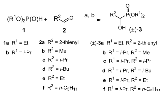
Scheme 1. Preparation of \alpha -hydroxyphosphonates ( \pm )- 3 . a) 1 and 0.16 equiv. of n -BuLi, THF, -78^\circ\text{C} , 30 min, then 2 , 1 h; b) \text{H}_2\text{SO}_4 . ( \pm )- 3a : 70%, ( \pm )- 3b : 75%, ( \pm )- 3c : 75%, ( \pm )- 3d : 74%, ( \pm )- 3e : 76%, ( \pm )- 3f : 90%.
