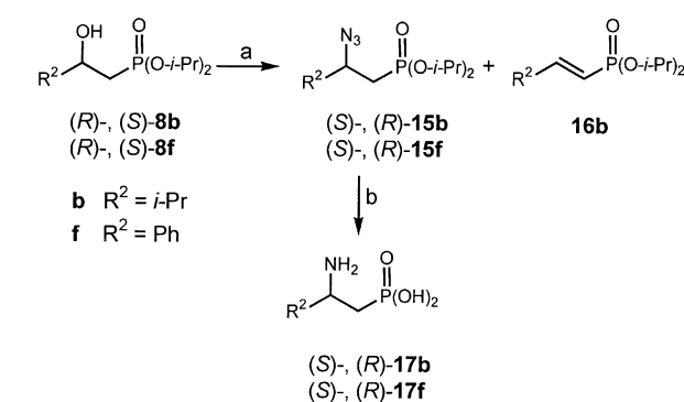
Scheme 10. Conversion of chiral, non-racemic \beta -hydroxyphosphonates 8 to \beta -aminophosphonic acids. a) \text{Ph}_3\text{P} , DIAD, \text{HN}_3 ; b) \text{Ph}_3\text{P} , \text{H}_2\text{O} ; 6 M HCl, reflux; Dowex 1, \text{AcO}^- .
