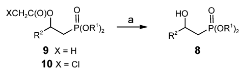
Scheme 5. Chemical hydrolyses of chiral, non-racemic \beta -acetoxyphosphonates 9. a) MeOH, \text{H}_2\text{O} , \text{Et}_3\text{N} .
