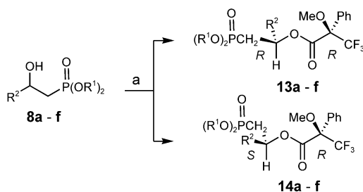
Scheme 9. Synthesis of ( R )-Mosher esters from \beta -hydroxyphosphonates 8 . a) ( S )-MTPA-Cl, pyridine, CH 2 Cl 2 , 18 h; H 2 O.
