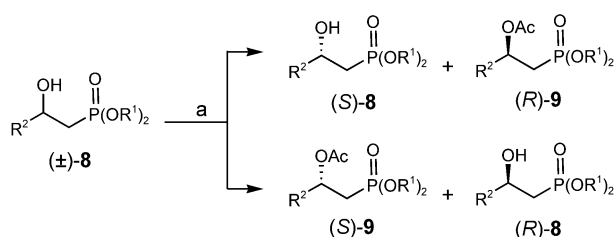
Scheme 4. Hydrolase-catalyzed acetylation of \beta -hydroxyphosphonates. a) Lipase or protease, isopropenyl acetate, t -BuOMe.
