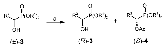
Scheme 2. Hydrolase-catalyzed acetylation of \alpha -hydroxyphosphonates. a) Lipase or protease, isopropenyl acetate, t -BuOMe.
